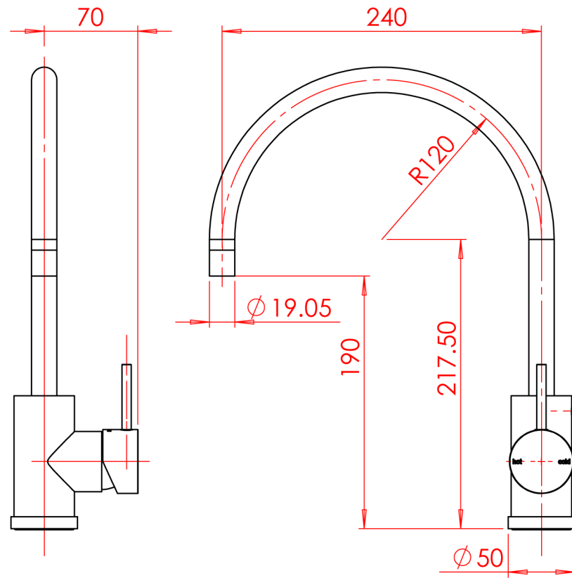
: LUCIA SIDE LEVER MIXER 240MM GOOSENECK
